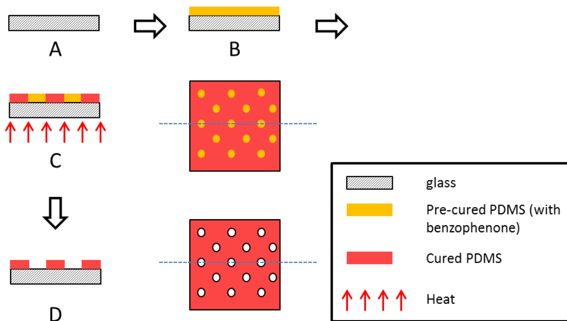
Figure 3.6: Schematic illustrations of fabrication procedures for molding PDMS. (A) A glass substrate. (B) Spin-coating pre-cured PDMS with benzophenone (like positive photoresist). (C) Exposing pre-cured PDMS under UV and baking at 110 °C for 3 minutes to cure the part that was not exposed. The schematic on the right represents the top view of the PDMS and the blue dash line corresponds to the cross-section area shown in the left. (D) Removing the uncured part of PDMS by toluene. The schematic on the right represents the top view of the PDMS and the blue-dashed line corresponds to the cross-sectioned area shown in the left.
