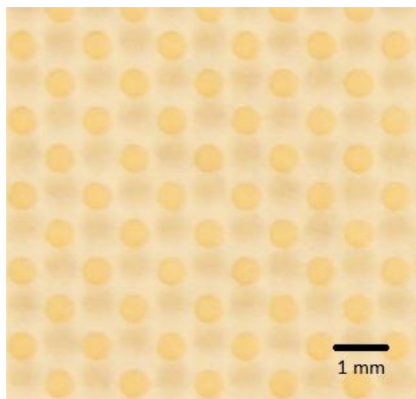
Figure 3.2: The top view photograph of AZ 40 XT photoresist-casted master mold. The diameters of the dots are 500\ \mu\text{m} , and the spacing between dots is 1\ \text{mm} . The depth of the master mold is 64\ \mu\text{m} .
